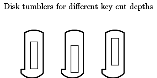
Figure 9.10: Workings of a disk tumbler lock
